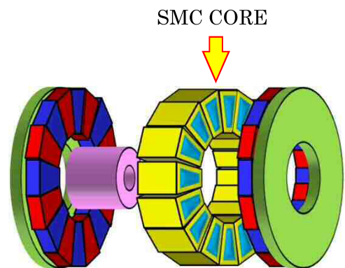
Usage example : Axial gap motor
